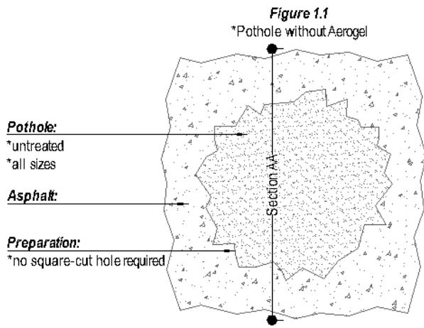
Figure 1: Pothole Aerogel Filling Process
